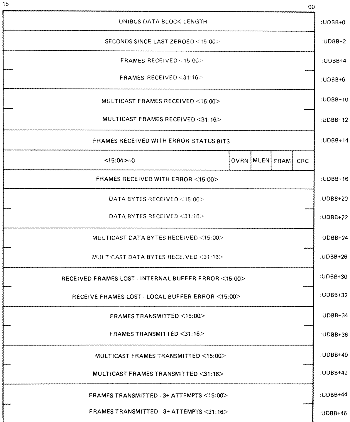
Figure 4-15 Read/Read and Clear Counters UDB Bit Format (Sheet 1 of 2)
