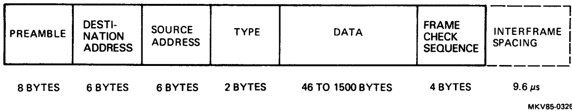
Figure 1-4 Format of a Data Frame
