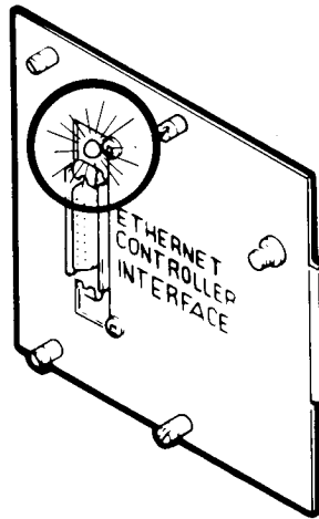
Figure 2-11 Bulkhead LED
