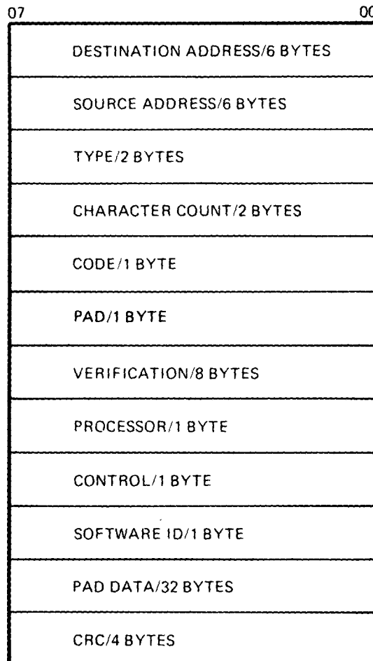
Figure 5-1 Boot Frame Format
