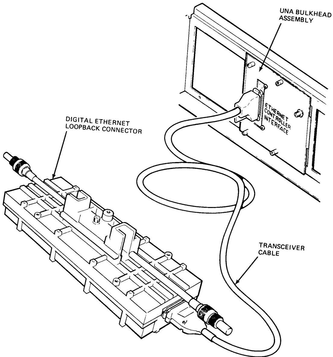
Figure 2-9 Loopback Transceiver Setup
