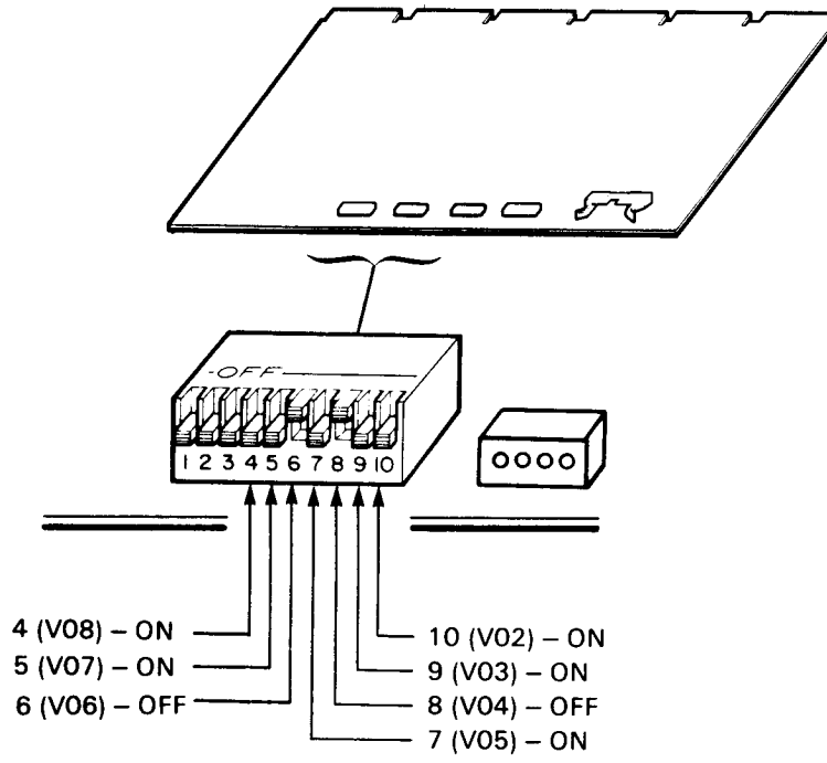
Figure 2-4 Switch Pack at E69, Vector Address Assignment
